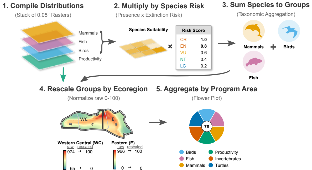
Figure 1: Overview of the MST methodology: species distribution models from the source datasets are merged, weighted by extinction risk scores (incorporating ESA, MMPA, MBTA, and IUCN protections), rescaled by ecoregion, and aggregated to management zones for visualization.
