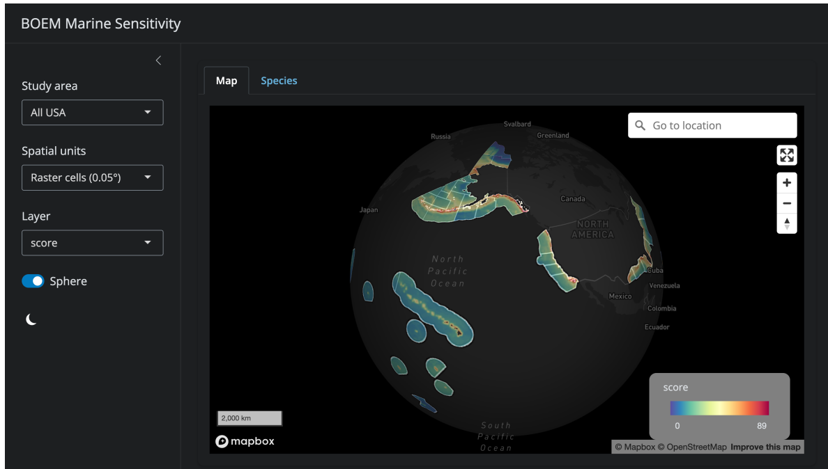
Figure B.1: The Scores application displaying cell-level sensitivity scores across US waters. The sidebar provides controls for study area selection, spatial resolution (raster cells vs. program areas), and layer choice. The globe view shows scores from 0 (blue) to 89 (red) with MapBox basemap.
