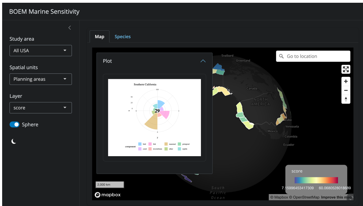
Figure B.2: The Scores application showing the flower plot panel for Southern California. Petal length represents each category's rescaled sensitivity score; petal width represents its weight. The center value (29) is the weighted mean across all categories.
