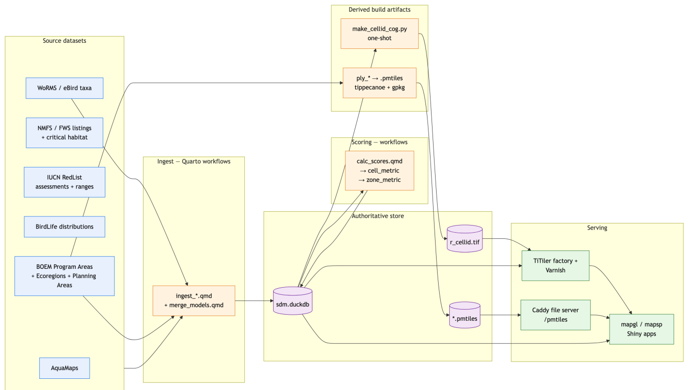
Figure 12.5: Data pipeline: ingest workflows populate DuckDB; scoring workflows compute cell_metric and zone_metric back into DuckDB; a one-shot COG regen and offline PMTiles build produce the derived artifacts the serving tier reads.
