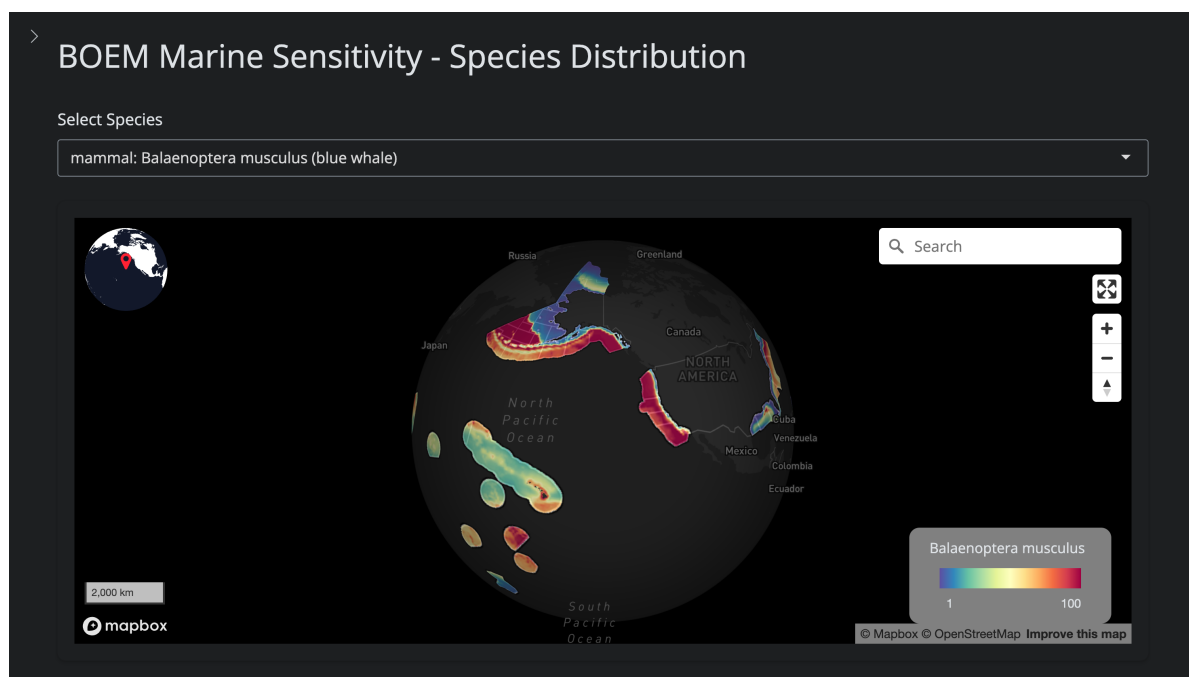
Figure D.1: The Species application showing the merged distribution model for blue whale ( Balaenoptera musculus ). Cell values range from 1 (low suitability) to 100 (high suitability). The species selector dropdown allows searching by common or scientific name with category prefix.
