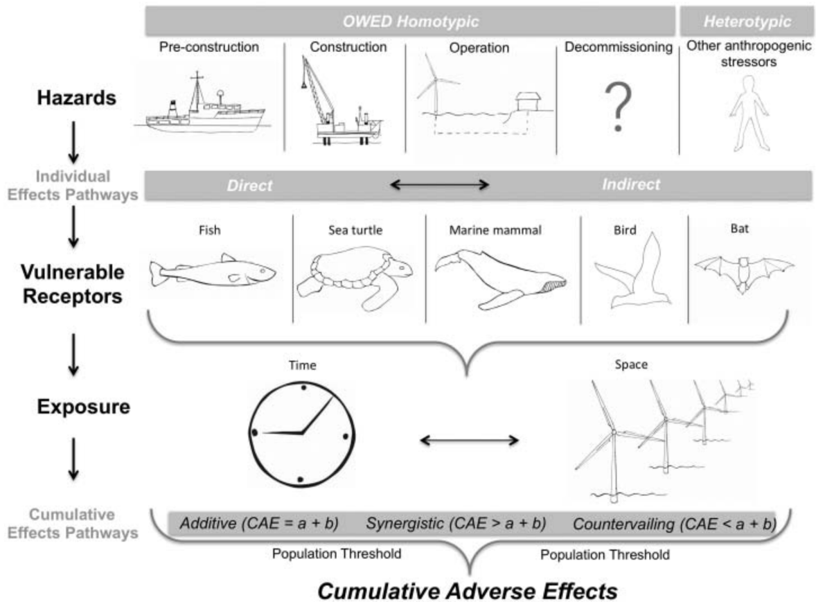
Figure 11.1: Cumulative adverse effects of offshore wind energy development on wildlife (Goodale and Milman 2016).
