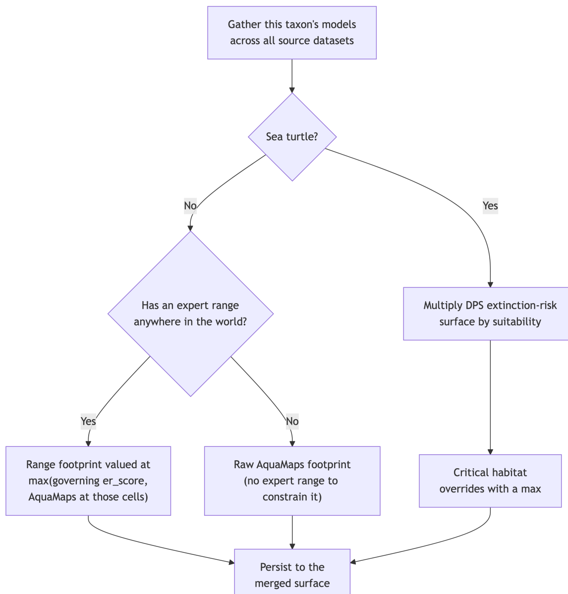
Figure 8.1: Merging one taxon's source models into a single surface.
