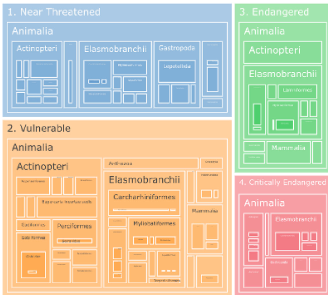
Figure 9.3: Treemap of species contributions to extinction-risk scores, organized by risk category and taxonomy.
