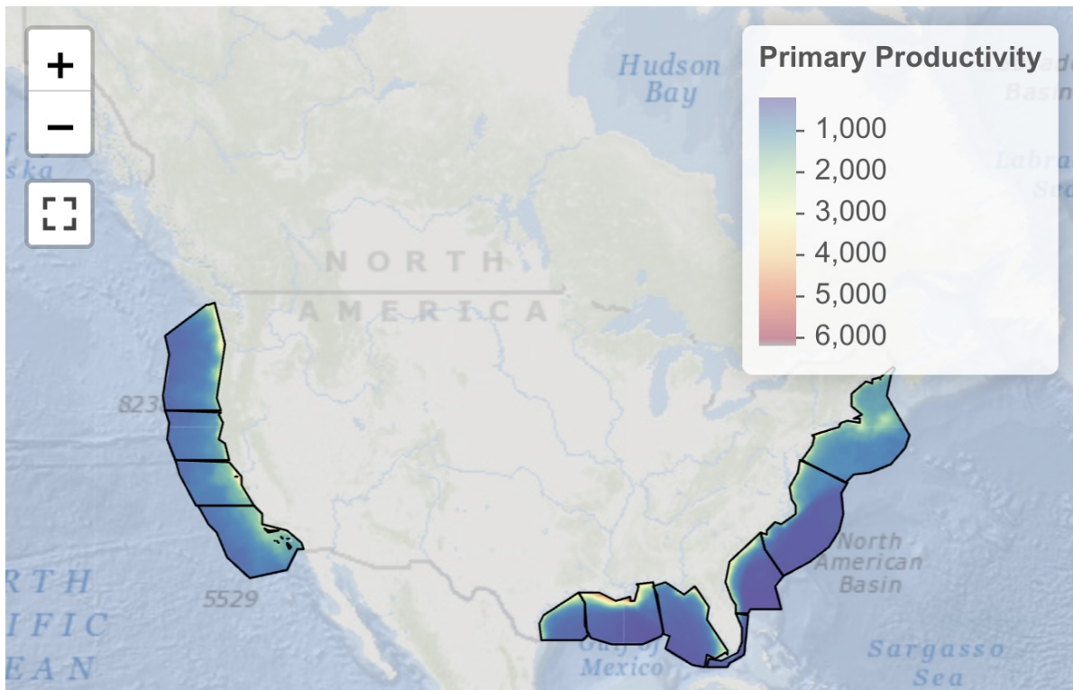
Figure 5.1: Primary productivity throughout the continental United States averaged across months of 2021, as measured by Oregon State’s Vertically Generalized Production Model (VGPM).
