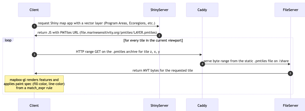
Figure 12.3: Sequence diagram: vector layers are served as static PMTiles archives through Caddy. Each tile is a byte-range read of the archive — no tile server process is in the path.
