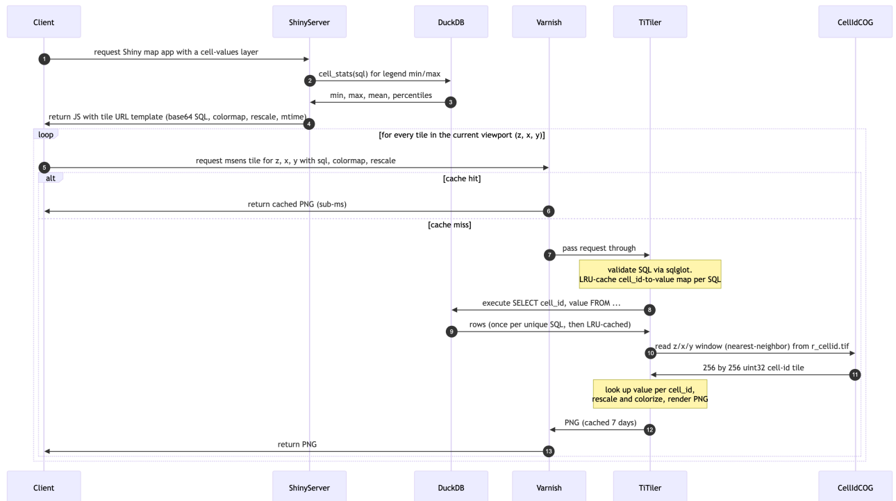
Figure 12.2: Sequence diagram: a cell-values raster layer is rendered on-the-fly by the custom msens TiTiler factory from the DuckDB source of truth. Varnish caches identical tile URLs for 7 days.
