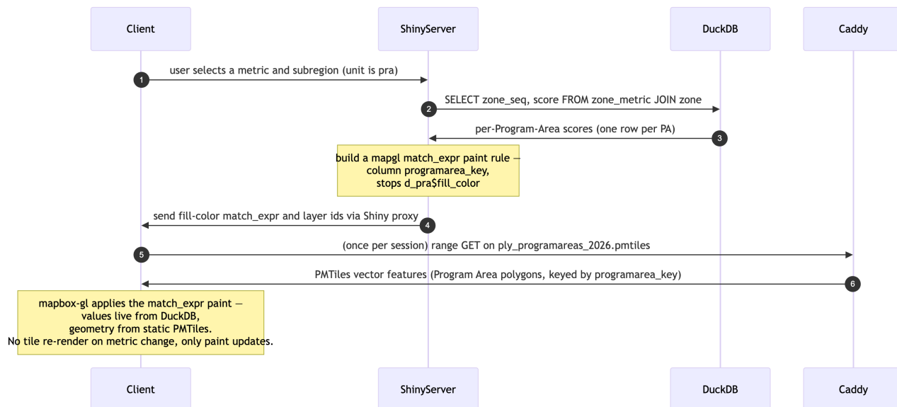
Figure 12.4: Sequence diagram: the Program Area choropleth. Polygon geometry is static (PMTiles from Caddy file server); per-area fill values come live from DuckDB's zone_metric table and are pushed into mapbox-gl's paint spec via a match expression. Switching metrics updates only the paint rule, not the tiles.
